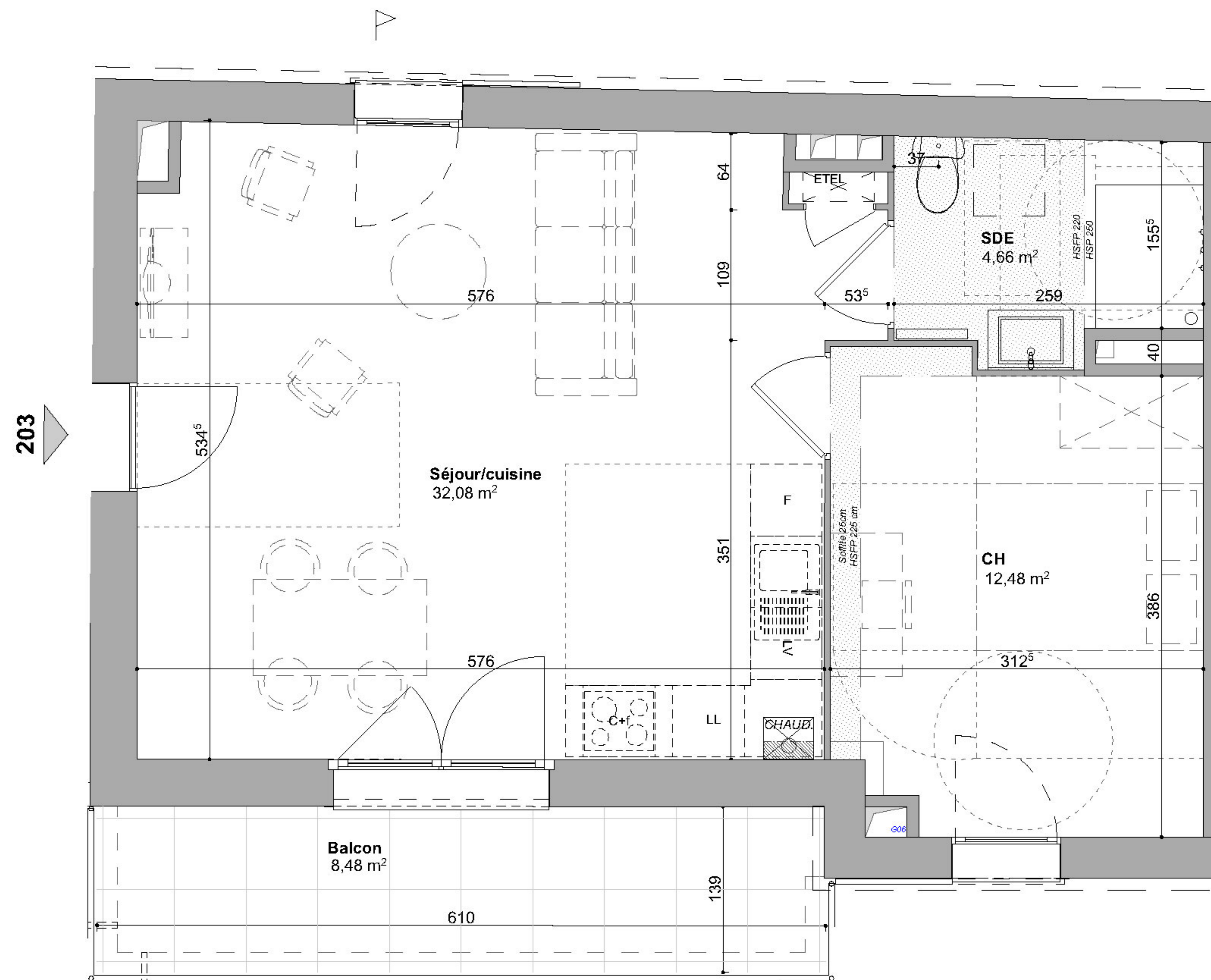
Plan - Ech: 1/50°
